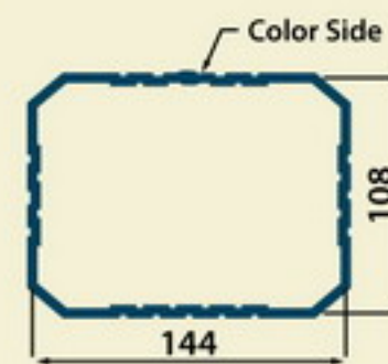
Downspout (0.6 mm)
